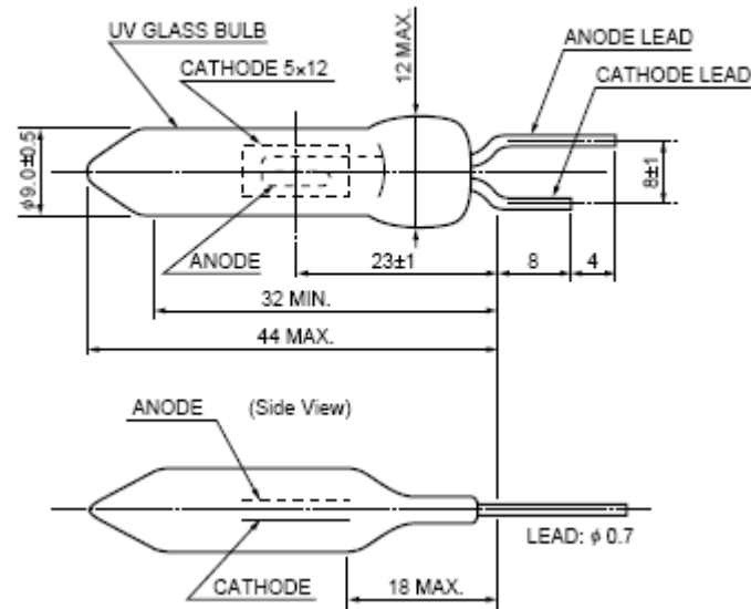
Figure 3: Dimensional Outline (Unit: mm)
